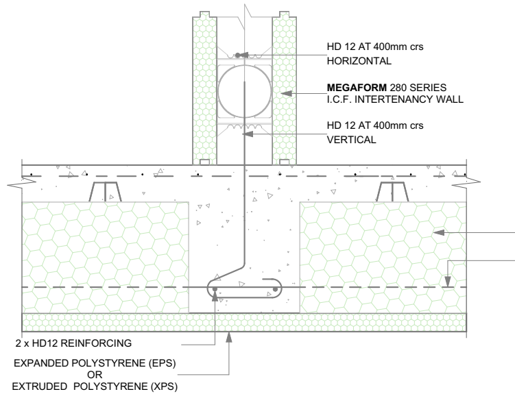
MEGAFOUND INTERNAL THICKENING WITH MegaForm 280 SERIES I.C.F. INTERTENANCY WALL
