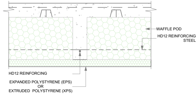
MEGAFOUND INTERNAL THICKENING
