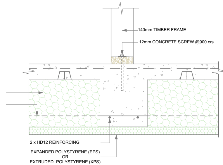
MEGAFOUND INTERNAL THICKENING WITH TIMBER FRAME INTERTENANCY WALL
