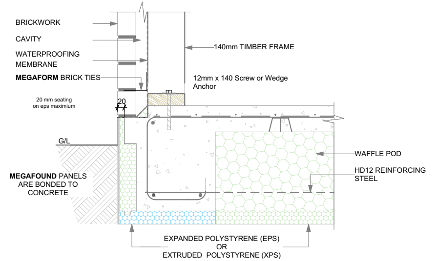
MEGAFOUND FULLY INSULATED FOUNDATION SYSTEMS WITH 140mm TIMBER FRAME AND BRICKWORK CLADDING
