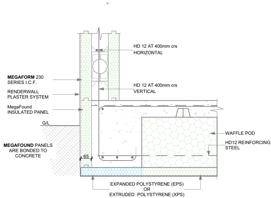
MEGAFOUND FULLY INSULATED FOUNDATION SYSTEMS WITH MEGAFORM I.C.F 230 SERIES
