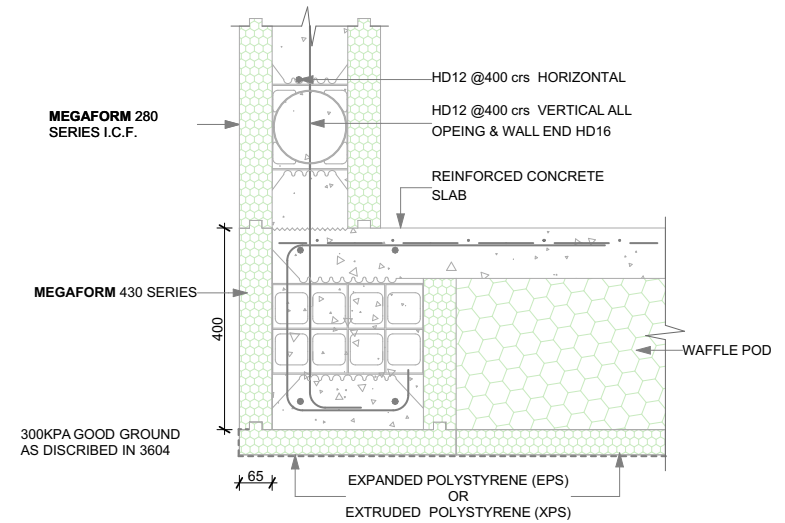
FULLY INSULATED MEGAFORM 430 SERIES AND MEGAPOD FOUNDATION SYSTEMS WITH MEGAFORM I.C.F 280 SERIES WALL
