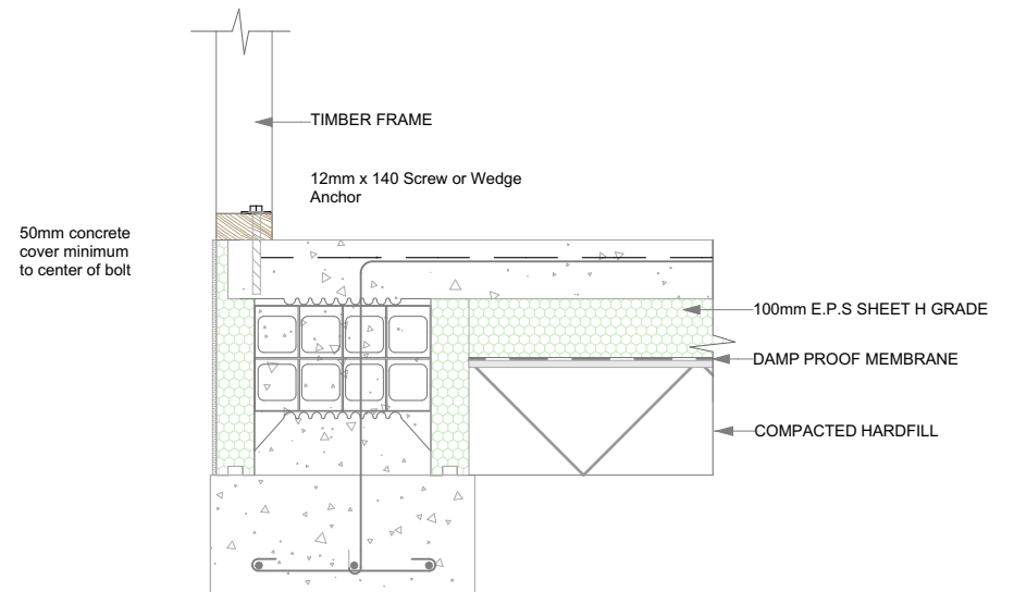
MEGAFORM FOUNDATION 430 SERIES WITH 90mm TIMBER FRAME
