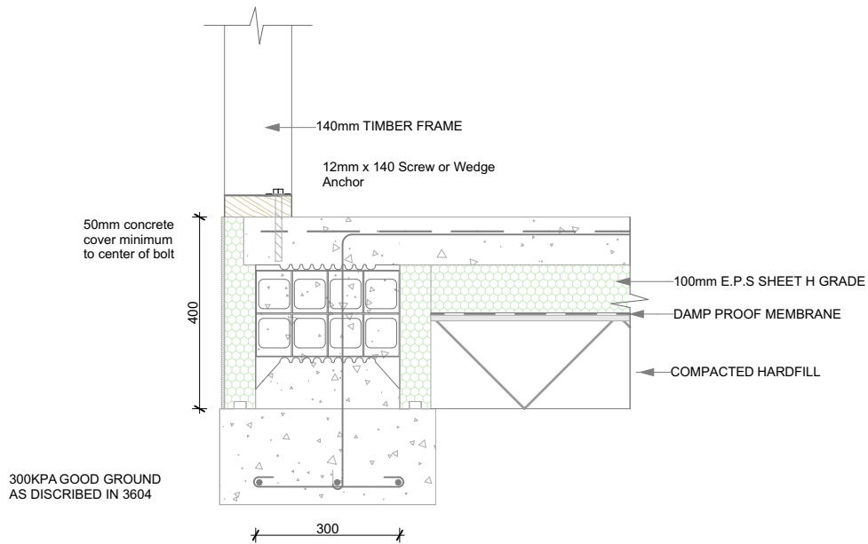
MEGAFORM FOUNDATION 430 SERIES WITH 140mm TIMBER FRAME
