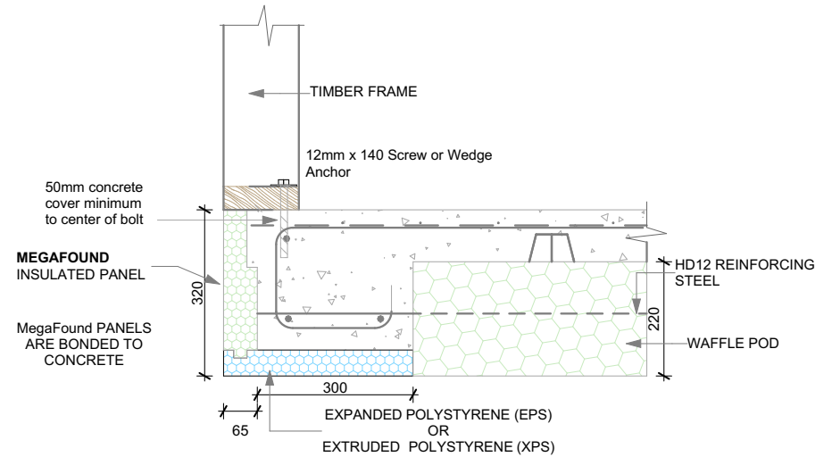
MEGAFOUND FULLY INSULATED FOUNDATION SYSTEMS WITH 140mm TIMBER FRAME CLAD EXTERNAL WALL
