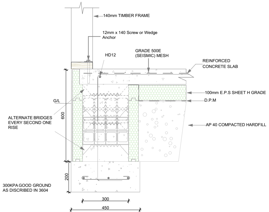
MEGAFOUND 430/600 HIGH FOUNDATION
