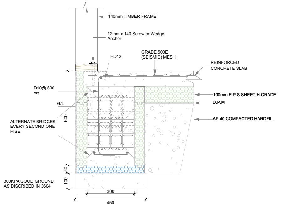
MEGAFOUND 430/600 HIGH FULLY INSULATED FOUNDATION
