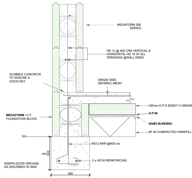
TYPICAL MEGAFORM FOUNDATION DETAIL WITH 330 SERIES COMPLIES 3604 2011
