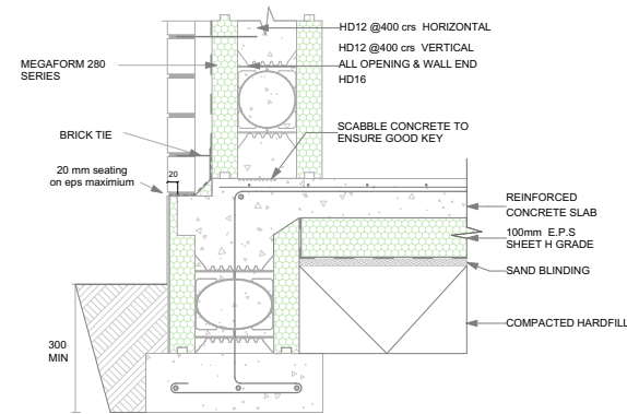
MEGAFORM FOUNDATION 330 SERIES WITH BRICKWORK AND MEGAFORM 280 SERIES BLOCK WALLCLADDING
