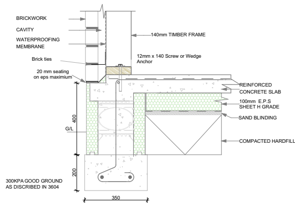
TYPICAL MEGAFORM FOUNDATION DETAIL WITH 140mm TIMBER FRAME
