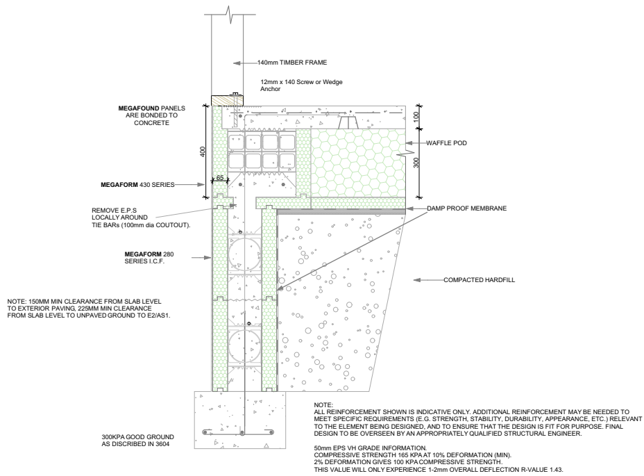
MEGAFOUND FULLY INSULATED WITH FOUNDATION WALL
