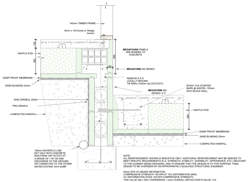
MEGAFOUND FULLY INSULATED STEPPED FOUNDATION
